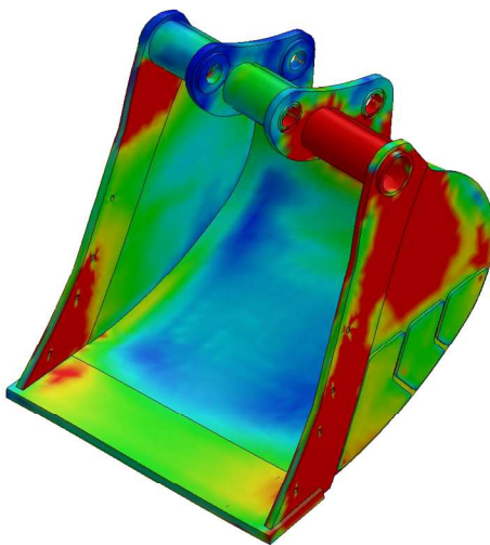
FEA ANALYSIS FOR STRESS TEST
